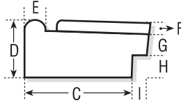
HEARTH FRONT SIDE VIEW
